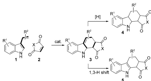
Scheme 1. Diels–Alder reaction of 3-vinyldioles 1 .
